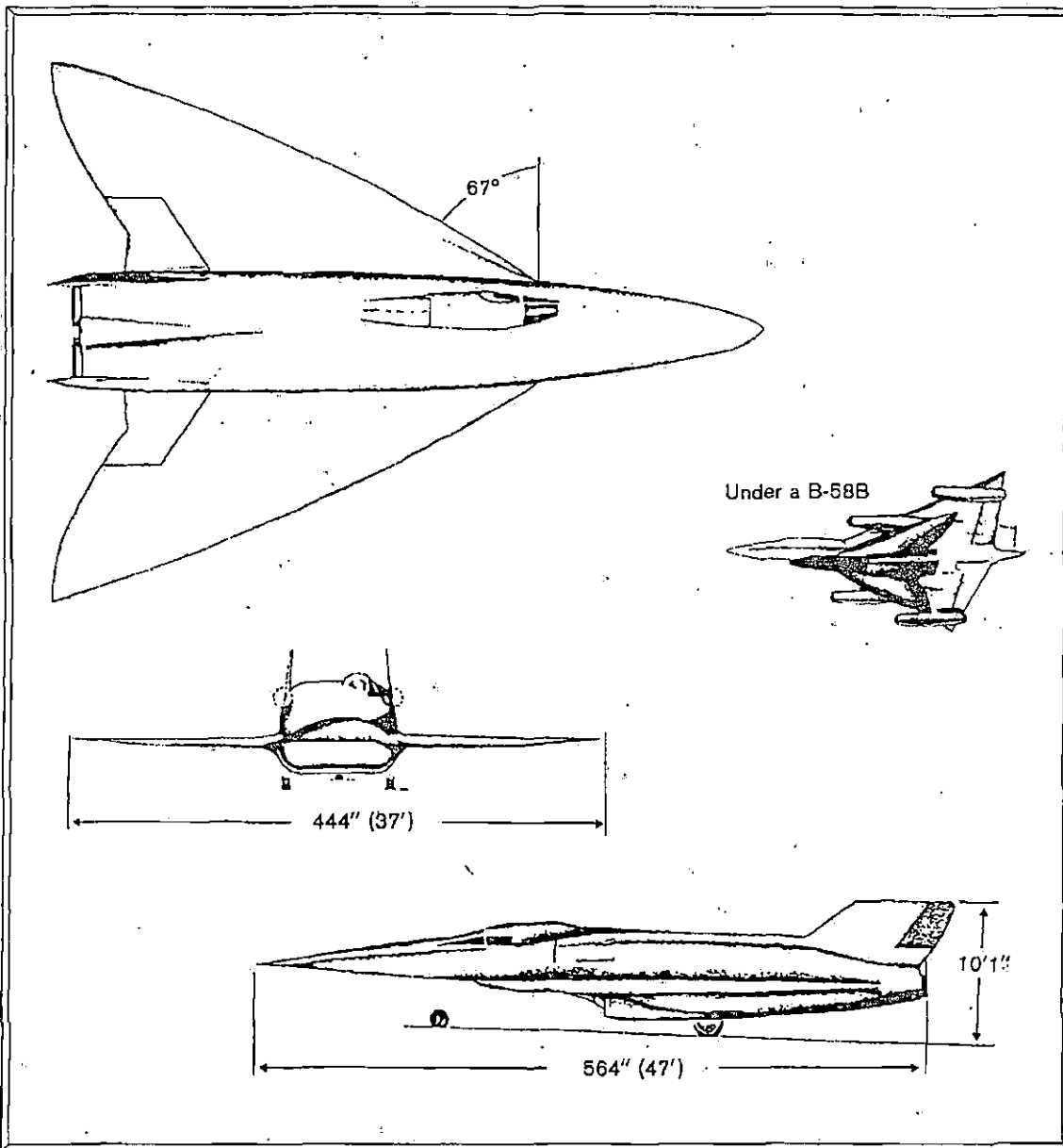
Convair FISH
