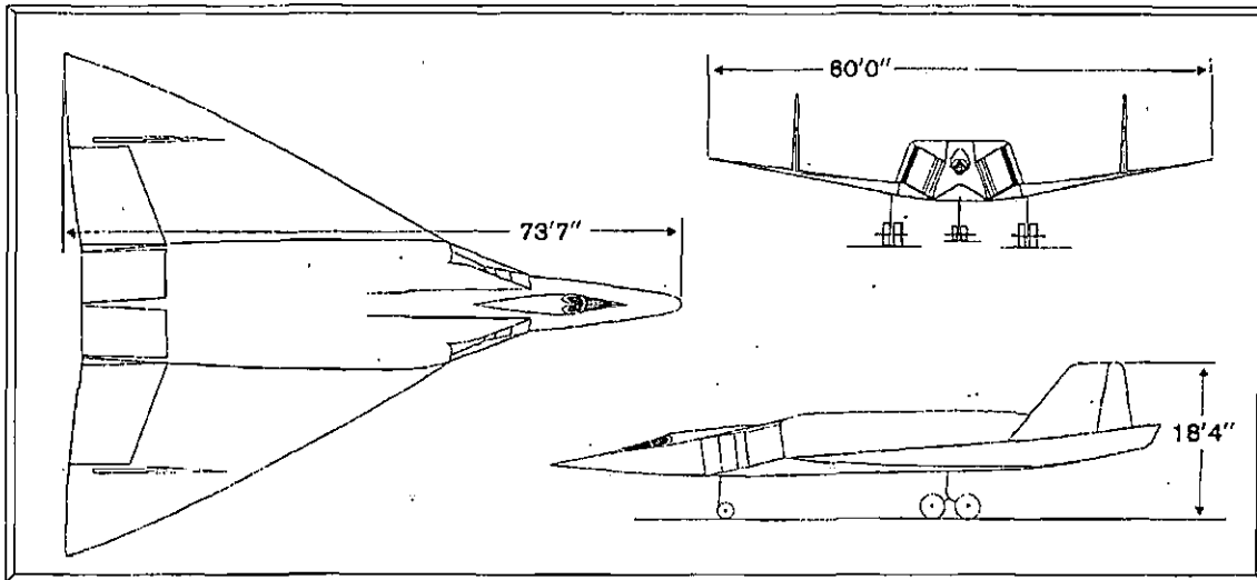
Convair KINGFISH
